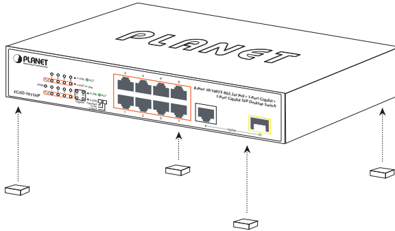
Figure 3-1: Attaching the Rubber Feet to the FGSD-1011HP
