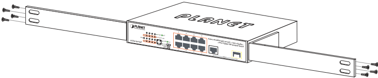
Figure 3-2: Attaching the Brackets to the FGSD-1011HP.
