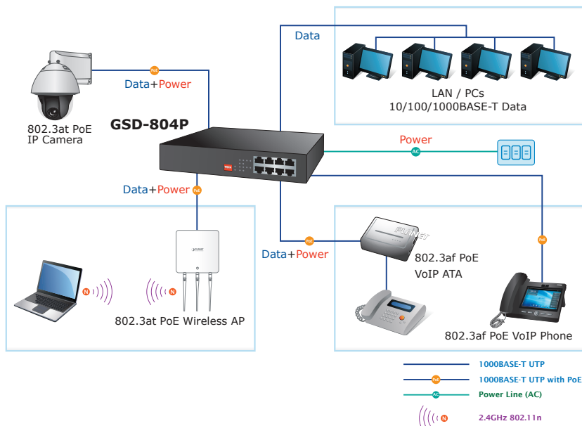
Figure 3-5: Department/Workgroup PoE/PoE+ Switch Connection
