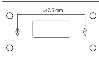
GDS-804P Switch Bottom Side
