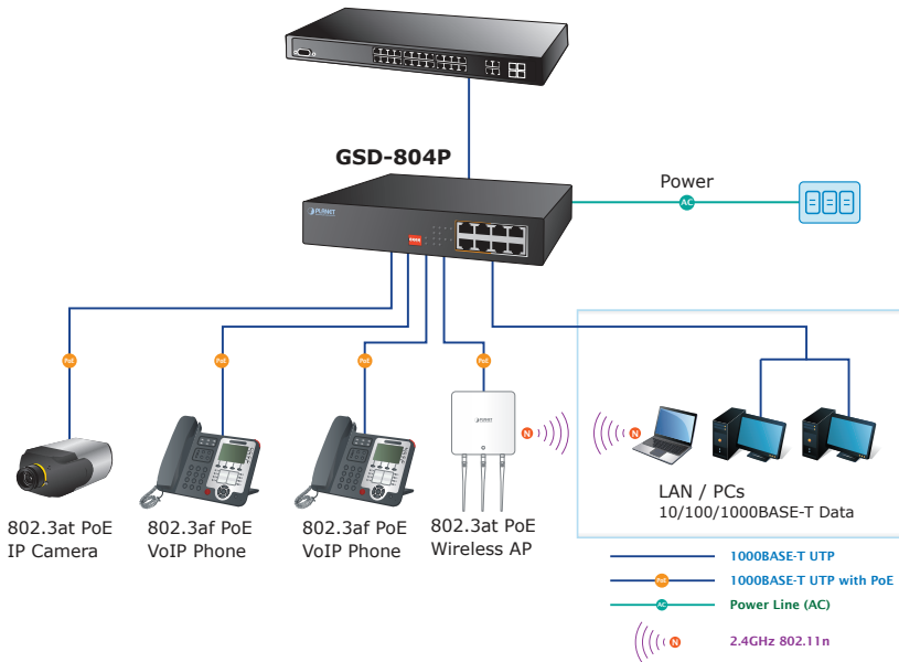
Figure 3-4: End node or Switch Connection
