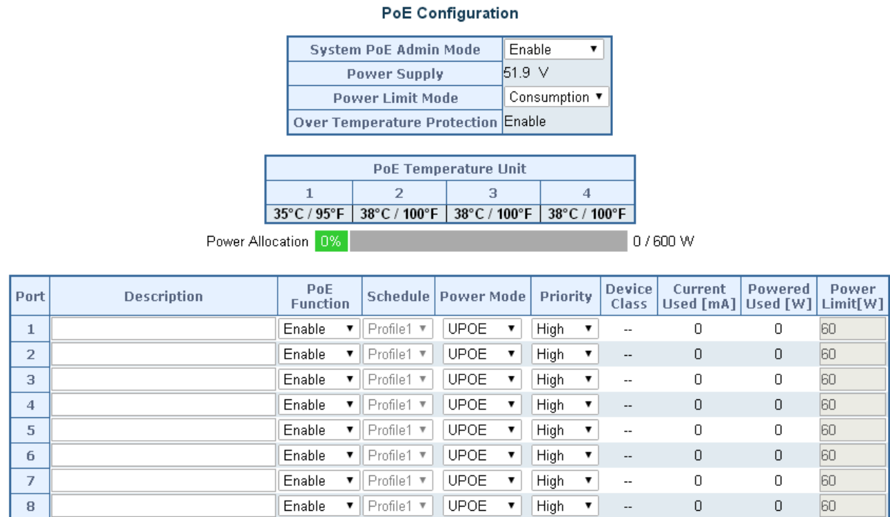
Figure 4-5-2: PoE Configuration Web Page Screen
