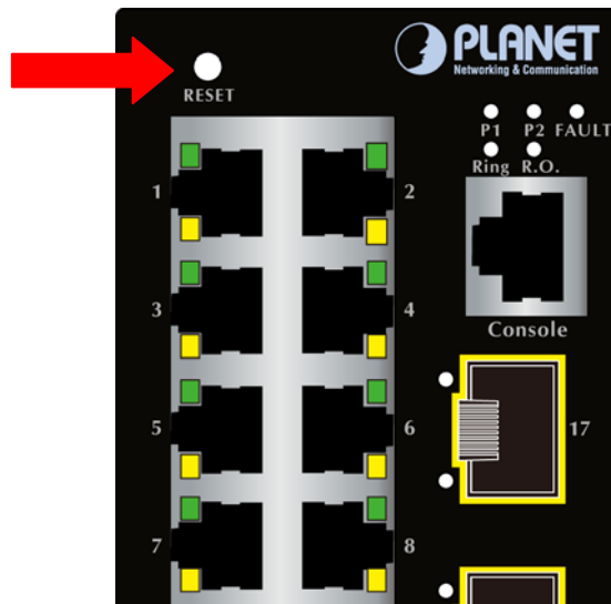
Figure 2-2: Reset button of Industrial Managed Switch
