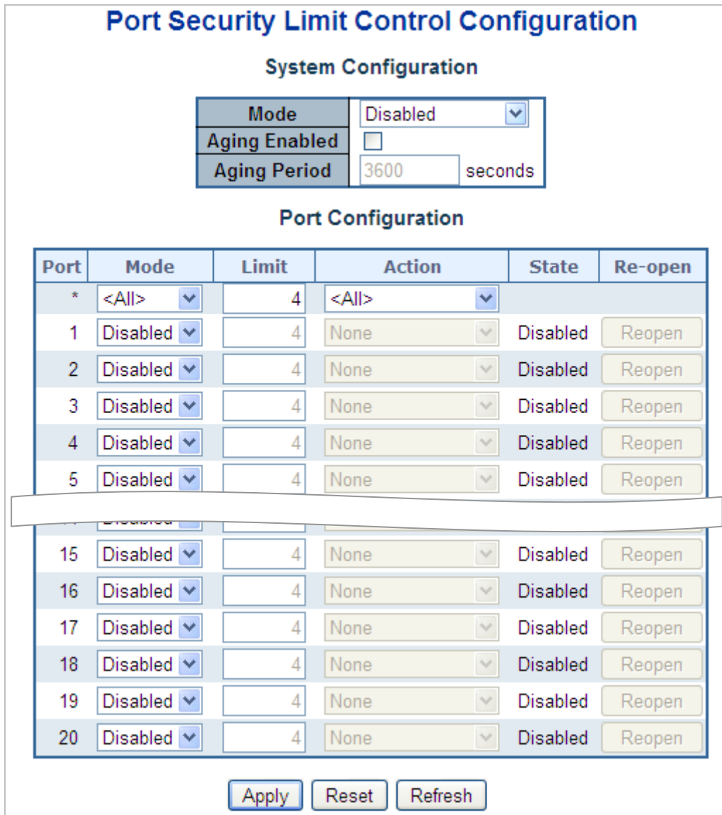
Figure 4-12-1: Port Limit Control Configuration Overview Page Screenshot
