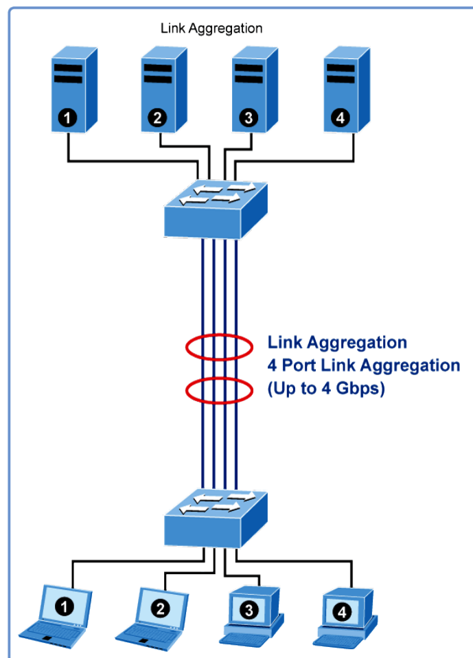
Figure 4-5-1: Link Aggregation
