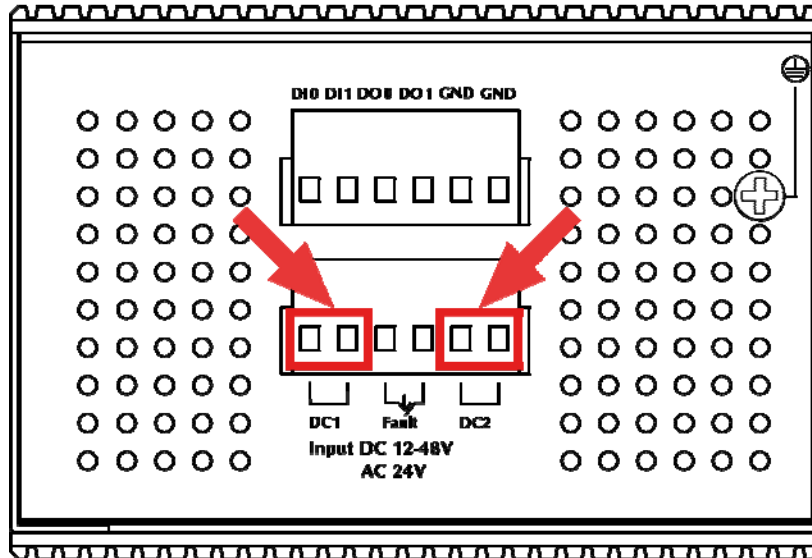
Figure 2-3: IGS-20040MT Upper Panel
