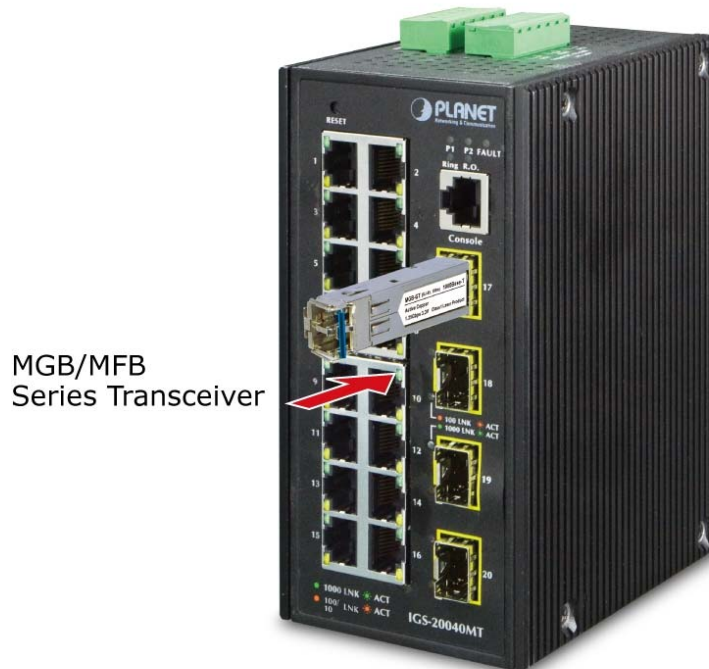
Figure 2-9: Plug-in the SFP Transceiver
