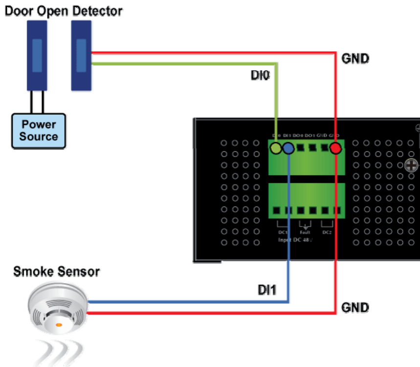
Figure 2-7 Wires DI0 and DI1 to Open Detector
