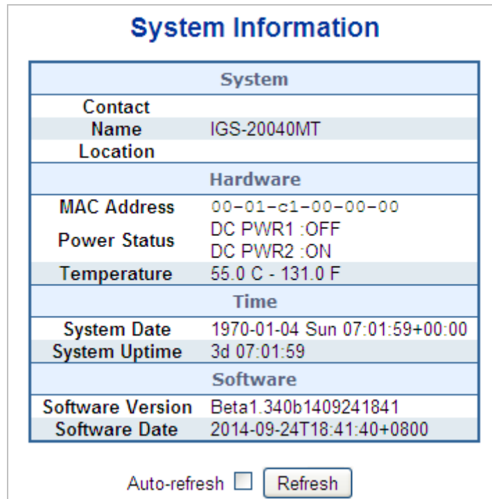
Figure 4-2-1: System Information Page Screenshot
