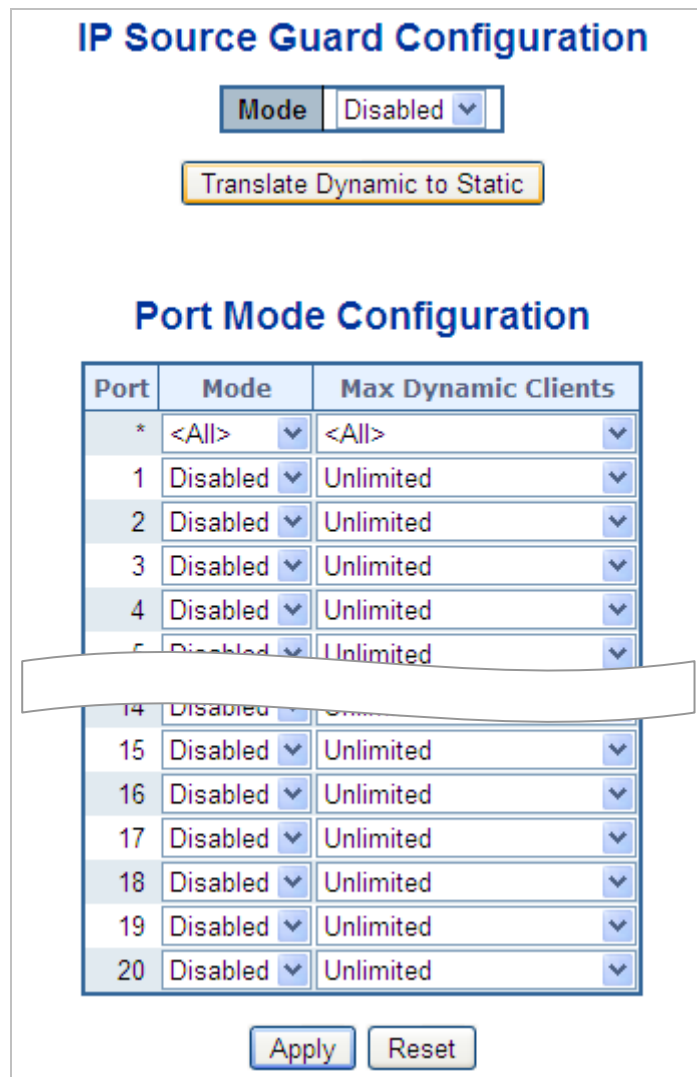
Figure 4-12-10: IP Source Guard Configuration Screen Page Screenshot
