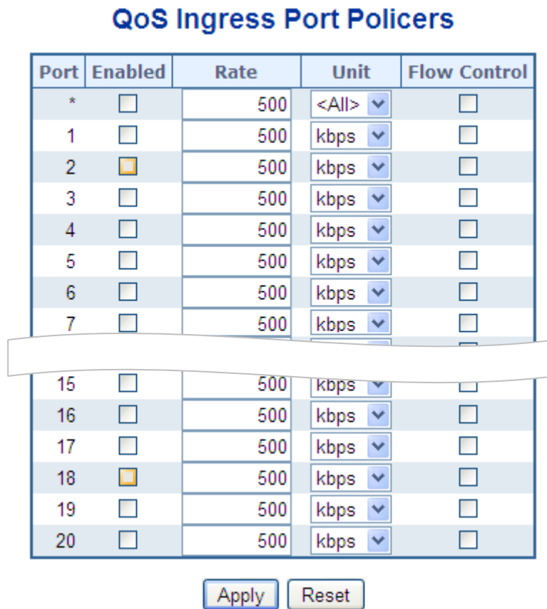
Figure 4-9-1: QoS Ingress Port Policers Page Screenshot
