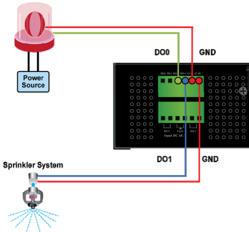
Figure 2-8 Wires DO0 and DO1 to Open Detector
