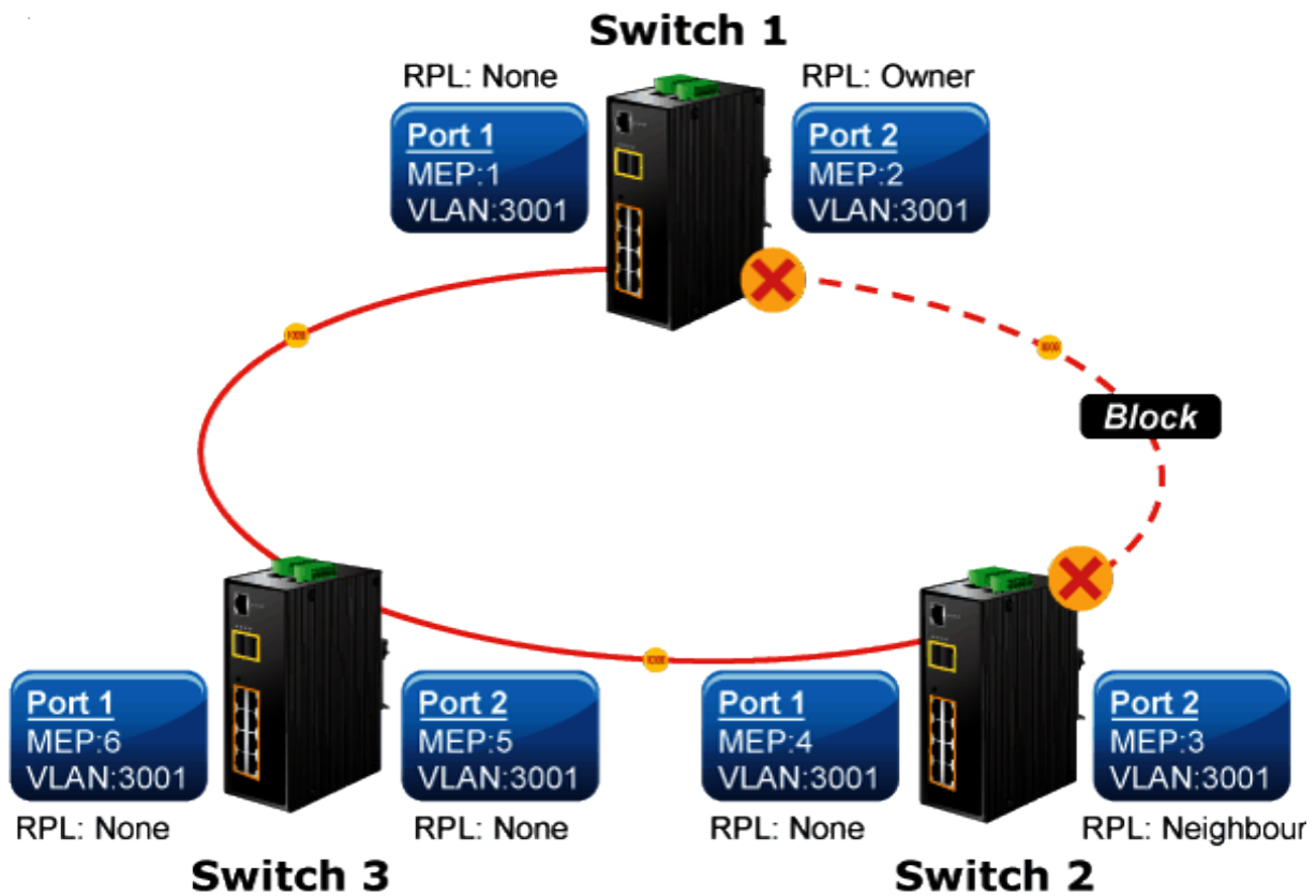
Figure 4-19-6: Ring Example Diagram
