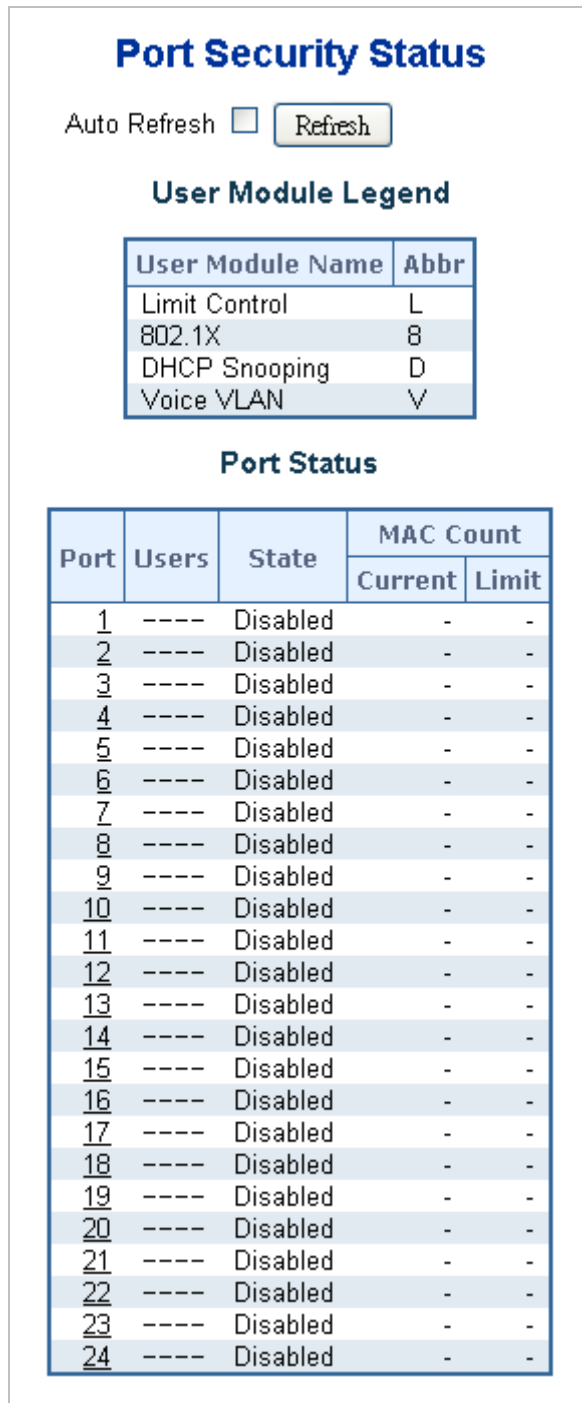
Figure 4-12-6 Port Security Status Screen Page Screenshot
