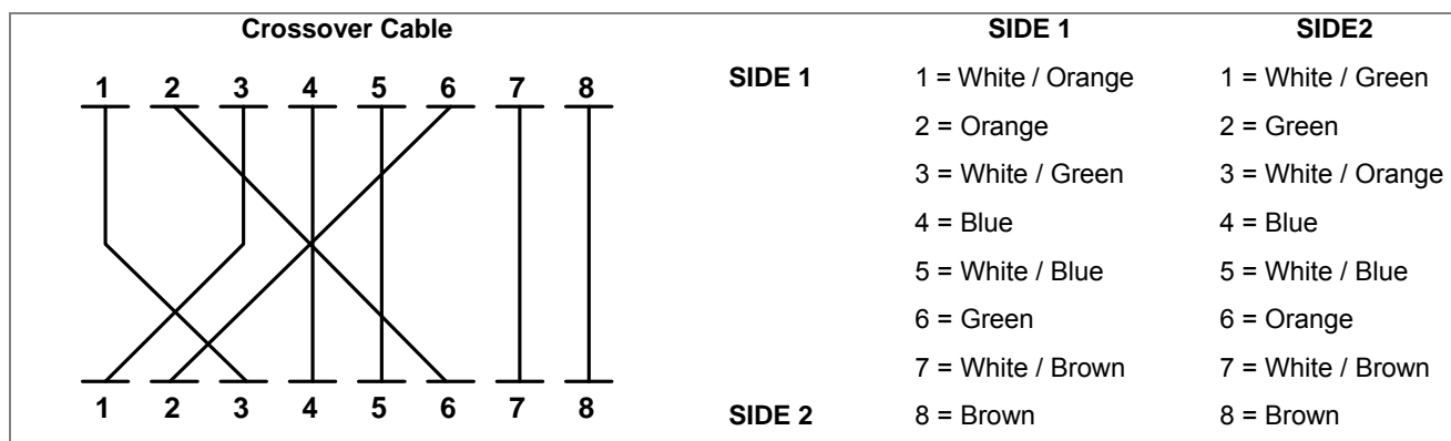
Figure A-1: Straight-Through and Crossover Cable
