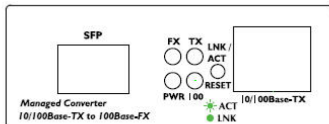
Figure 2-2 PLANET FT-905A Front Panel
