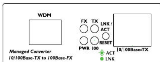
Figure 2-3 PLANET FT-906A20 / FT-906B20 Front Panel
