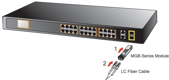
Figure 3-4: Plug In the SFP Transceiver
