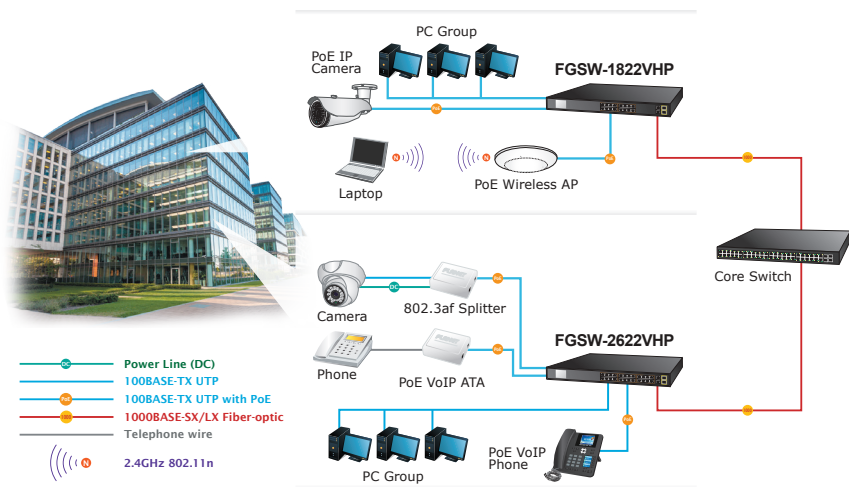
Figure 3-6: Two Different Networks Managed by One Control Center
