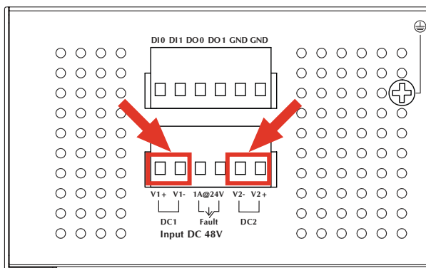
Figure 3-2: IGS-10020PT/IGS-10020HPT Upper Panel
