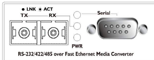
Figure 2-6 PLANET ICS-102 Front Panel
