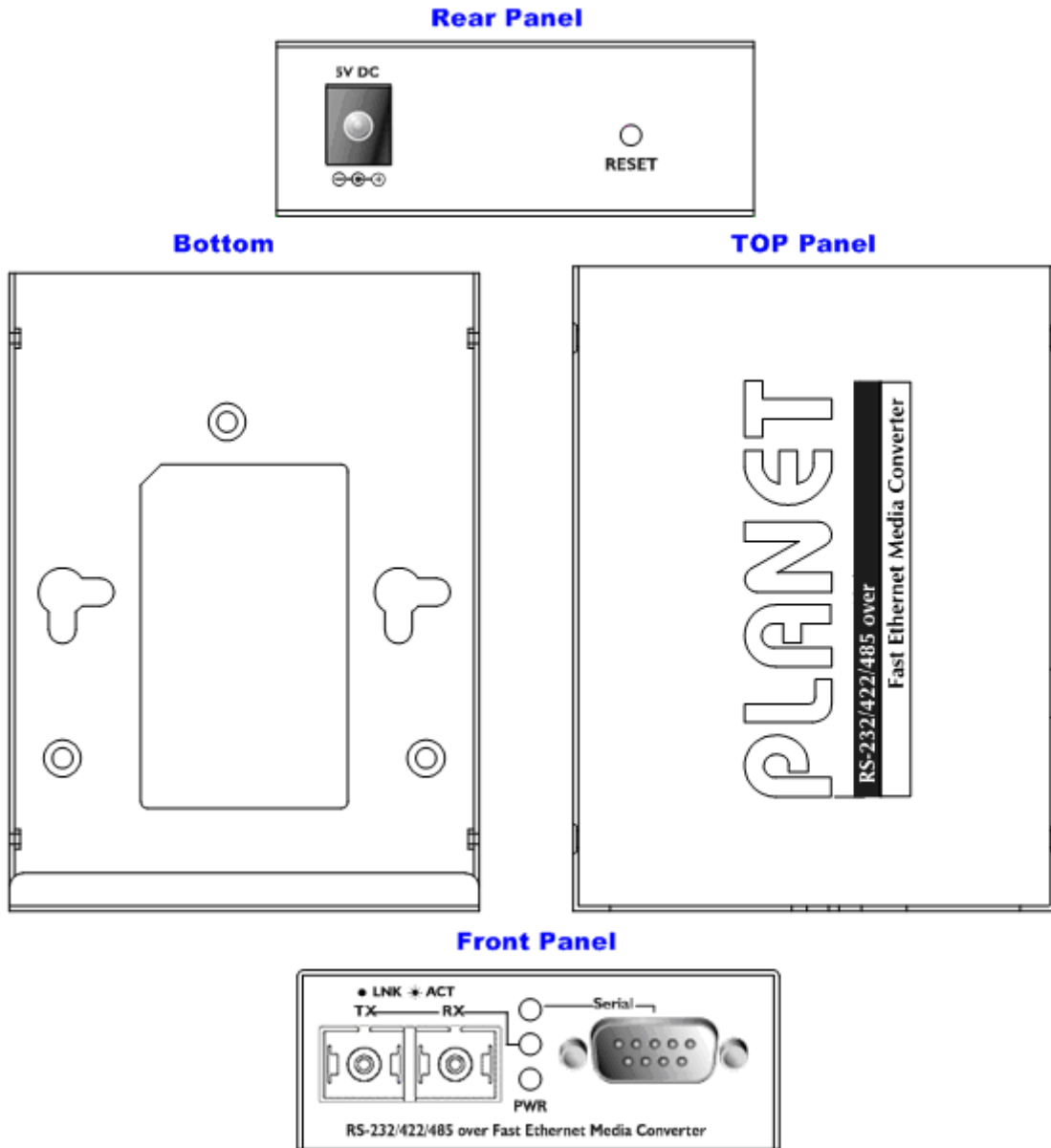
Figure 2-5 ICS-102 / ICS-102S15 panel layout
