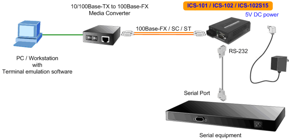
Figure 2-7 ICS-101 / ICS-102 / ICS-102S15 stand alone installation
