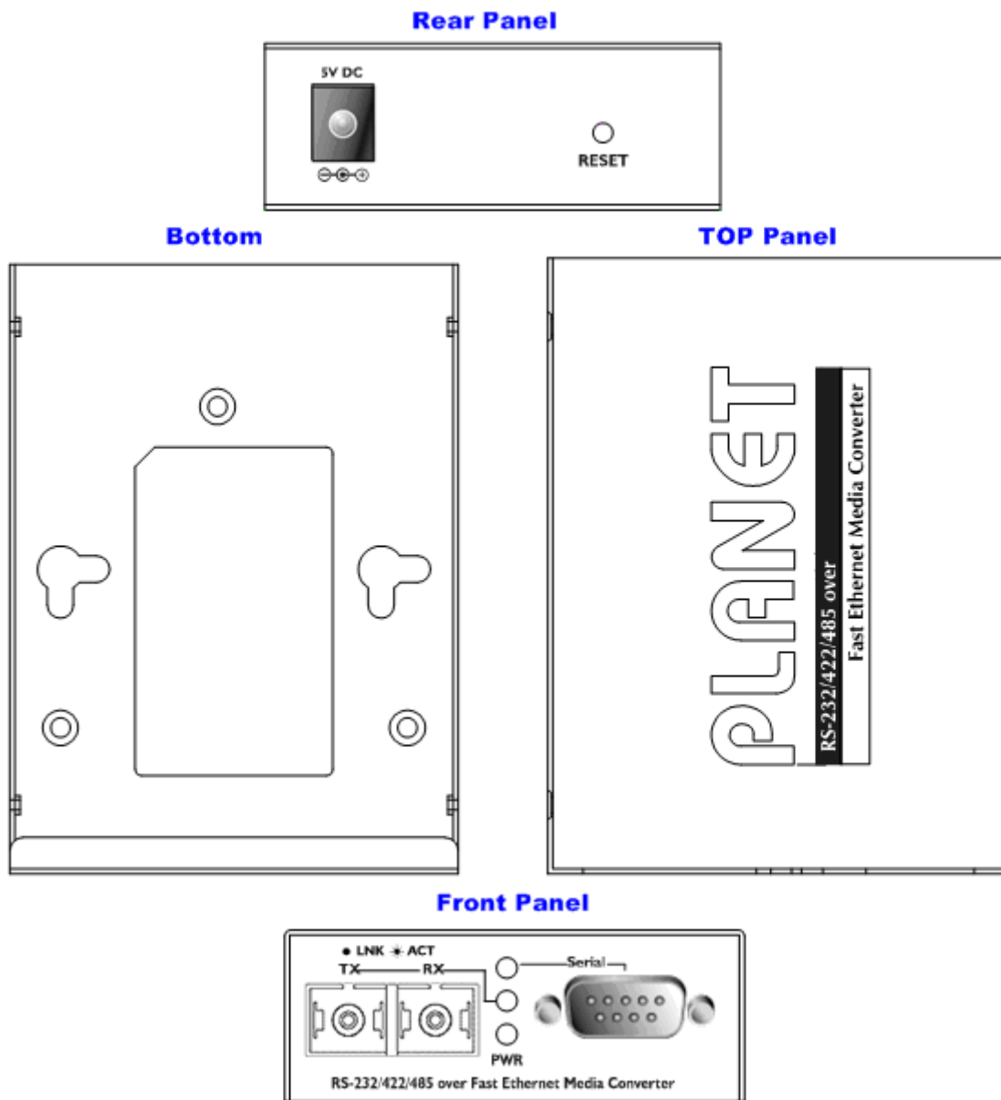
Figure 2-3 ICS-102 / ICS-102S15 panel layout
