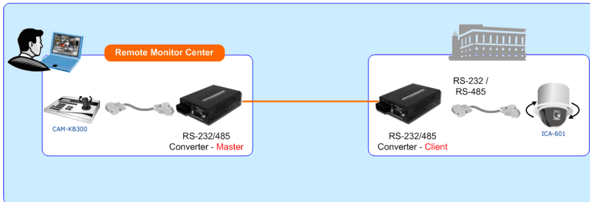
Figure 1-4 Serial Converter for Distance Extend Application
